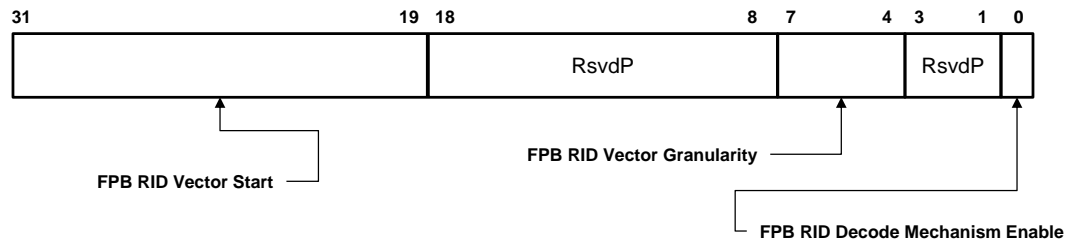
Figure 7-y3: FPB RID Vector Control 1 Register
