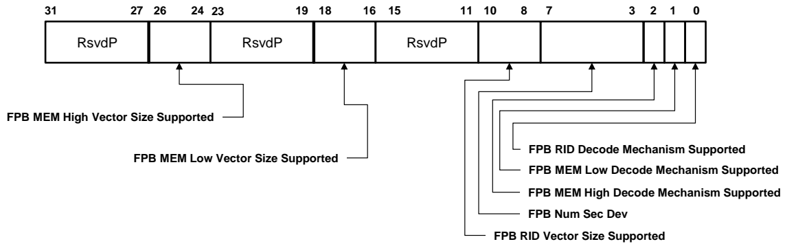
Figure 7-y2: FPB Capabilities Register
