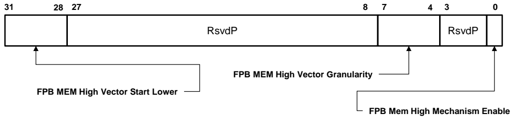
Figure 7-y6: FPB MEM High Vector Control 1 Register
