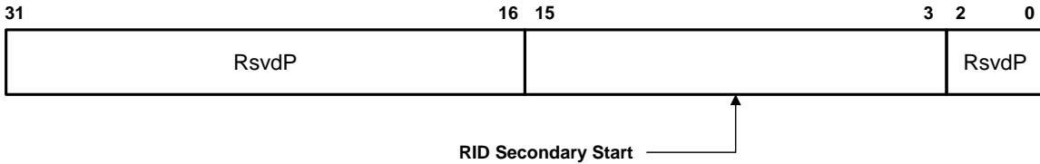
Figure 7-y4: FPB RID Vector Control 2 Register
