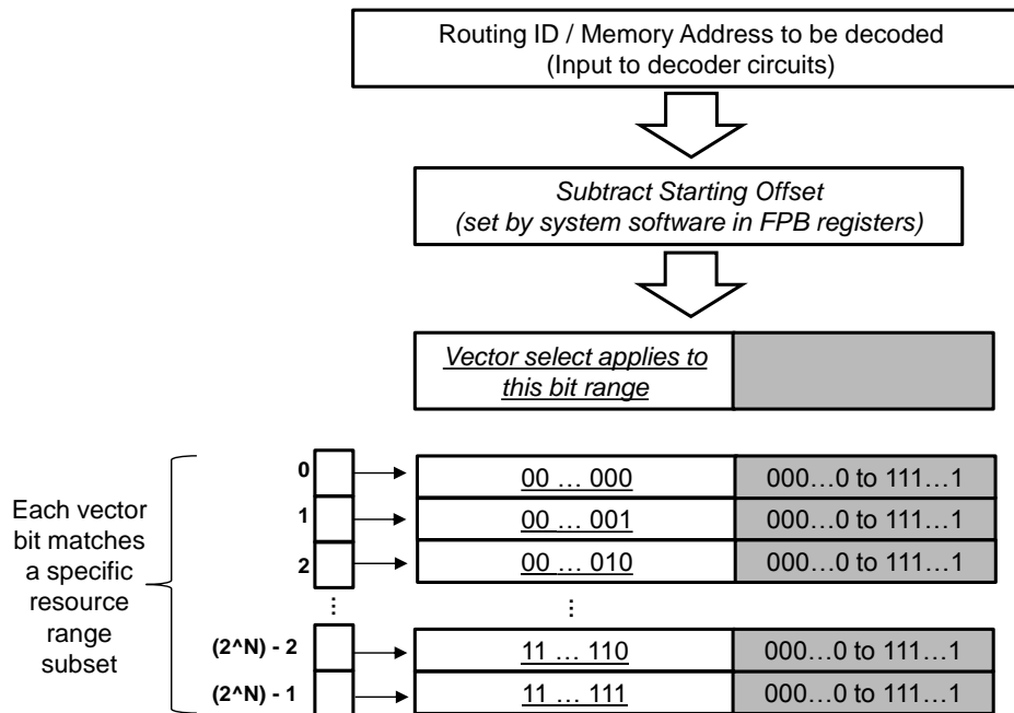
Figure 6-x1b: Vector Mechanism for Address Range Decoding
